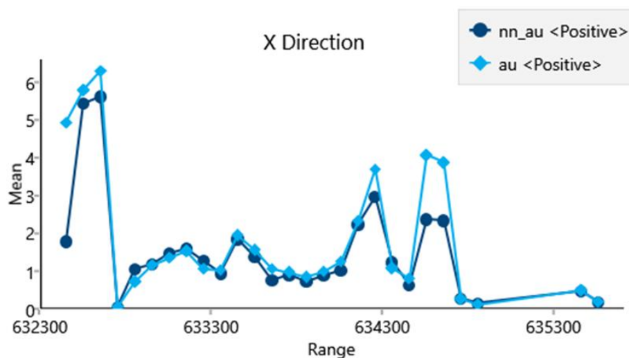
Figure 14-6: Drift Analysis for Palito Mine (x direction)
