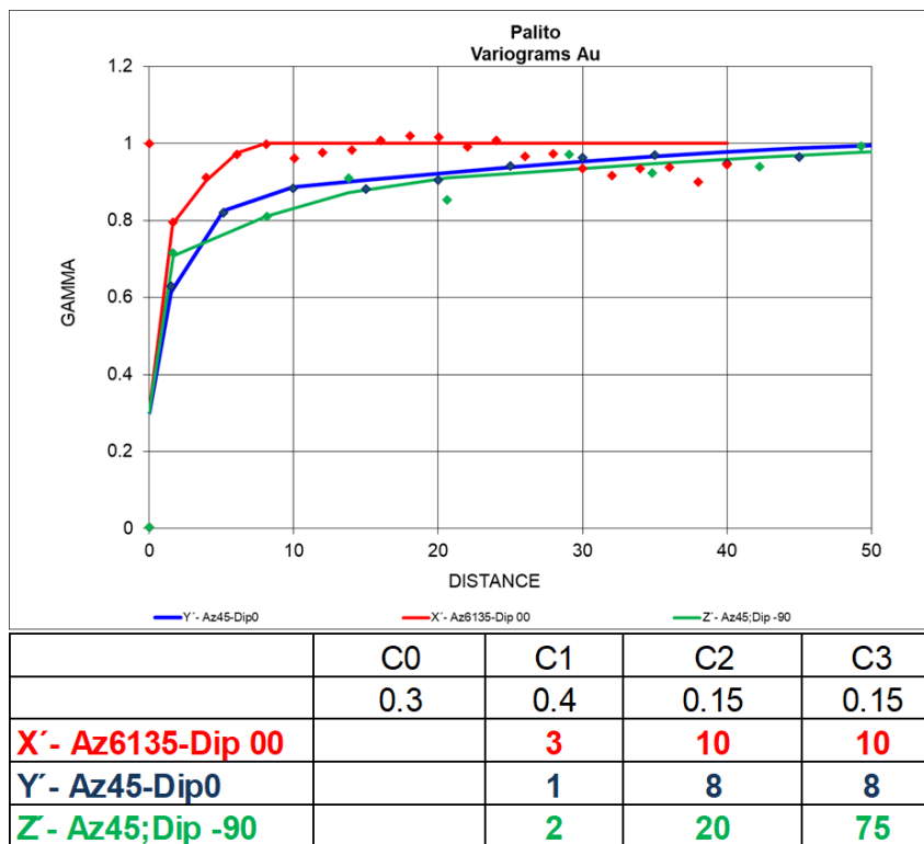
Figure 14-5: Variograms and structures definition for Palito Mine
