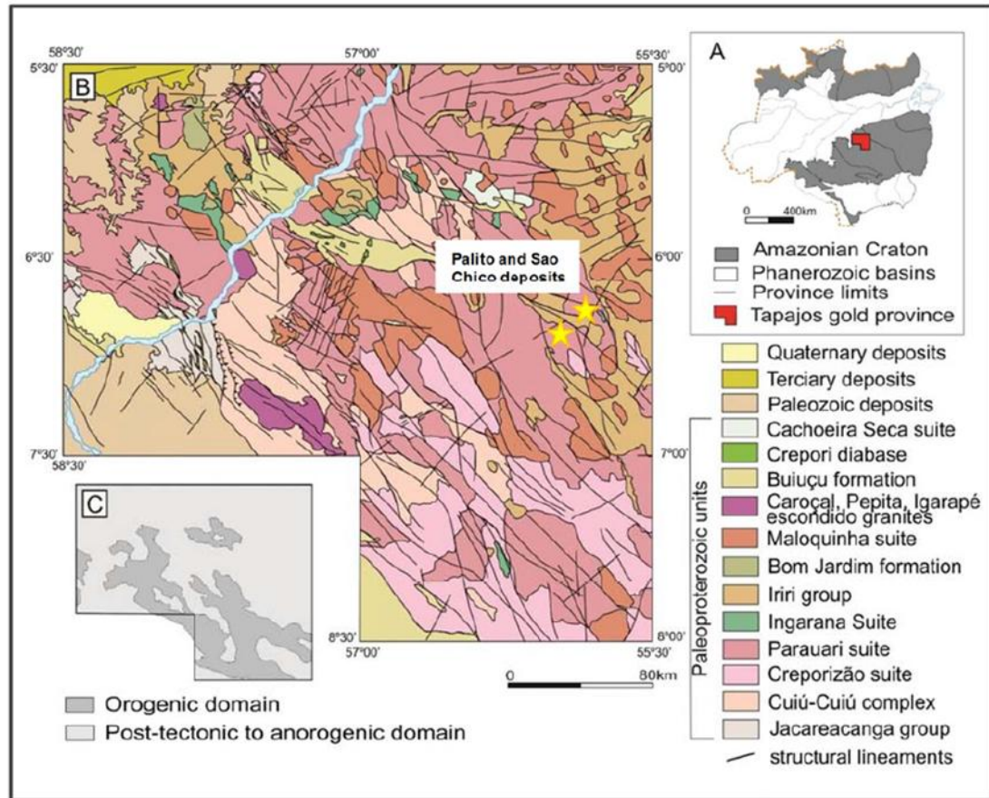
Figure 7-1: Regional Geology Setting with Palito and São Chico Deposits Hosted Within the Paleoproterozoic Paráuari Suite
