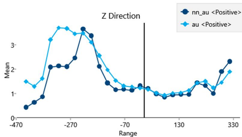
Figure 14-8: Drift Analysis for Palito Mine (vertical)
