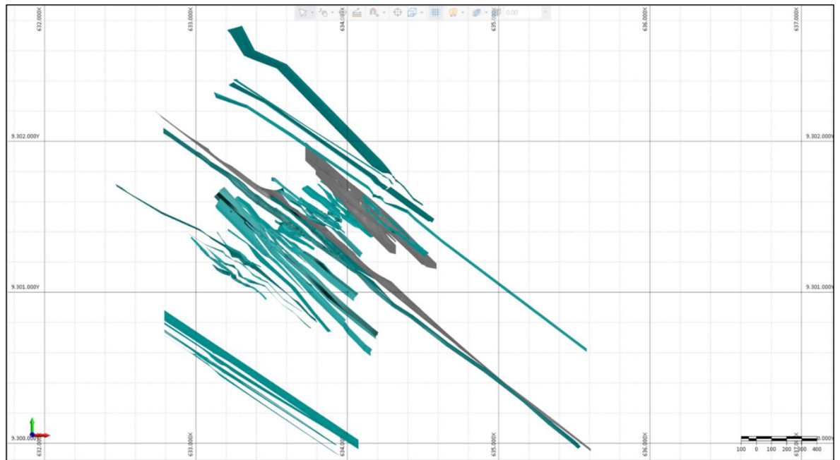
Figure 14-3: Plan View of Modelled veins in Palito Mine (44 veins total)
