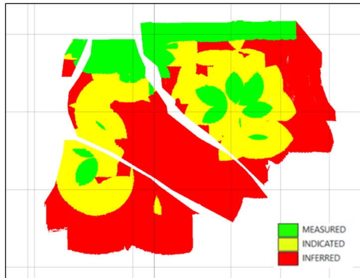
Figure 14-9: Longitudinal Section of IPE vein showing Classification
